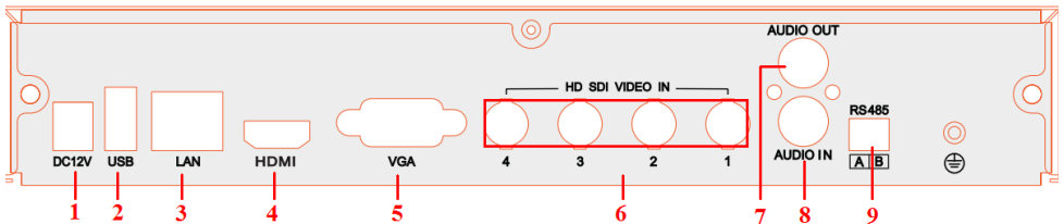
Fig 2-3 Rear Panel for 4-ch
