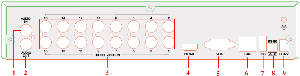
Fig 2-5 Rear Panel for 16-ch
