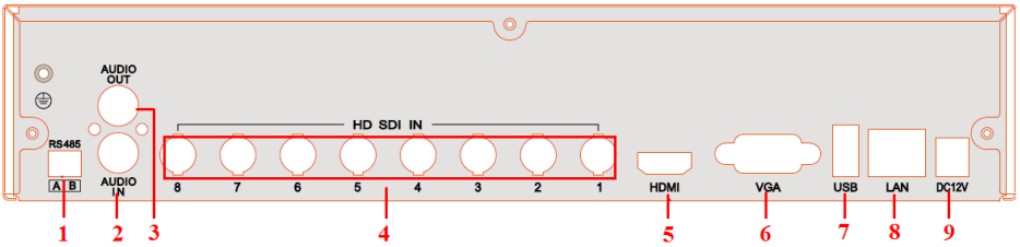
Fig 2-4 Rear Panel for 8-ch
